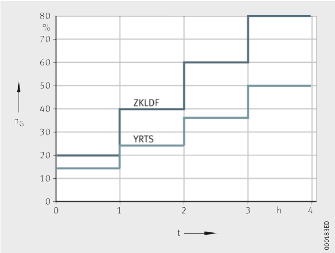
Figure 13 Running-in cycle for initial operation and after overlubrication
