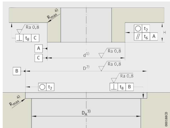
Figure 14 Requirements for the adjacent construction, YRT, YRTS, ZKLDF
