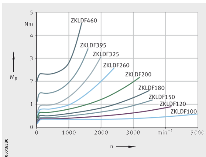
Figure 11 Frictional torques as guide values for ZKLDF, statistically determined values from series of measurements
