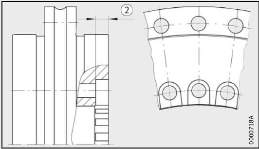
Screw counterbore open 5) Bearing inside diameter unsupported in area 2
