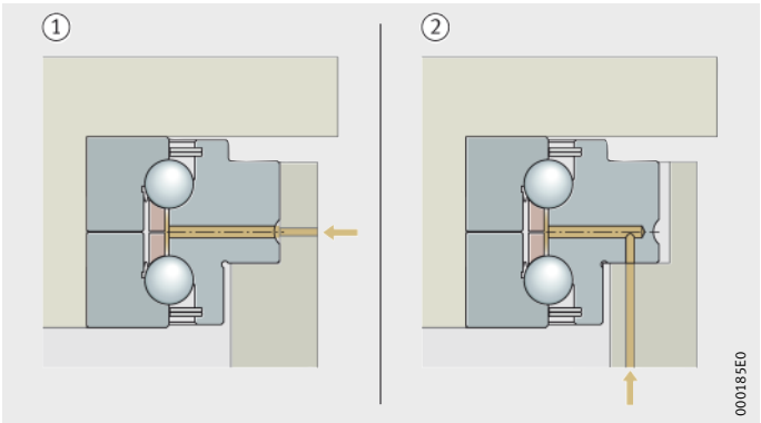
Figure 12 Options for relubrication
