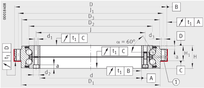
ZKLDF 1 Contact surface/centring diameter
