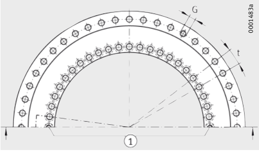
Hole pattern 1 Two retaining screws
