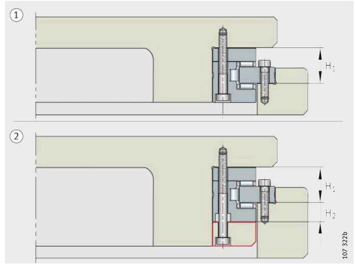
Figure 16 Mounting variants
