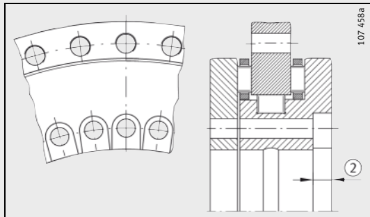
Screw counterbore open Bearing inside diameter unsupported in area 2
