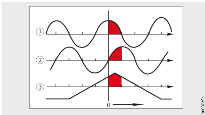
Figure 9 Reference signal position
