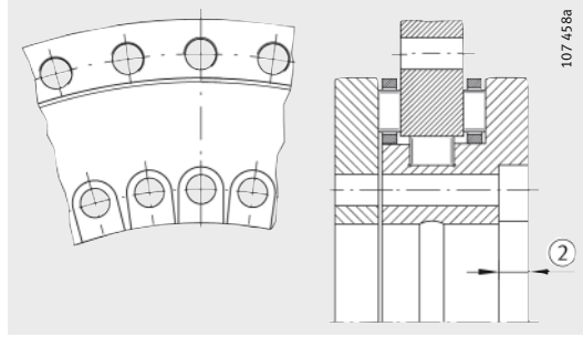
For YRT325: 2 Screw counterbores open 5)
