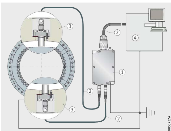
Figure 6 Shielding and post-processor
