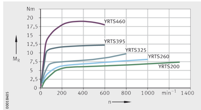
Figure 10 Frictional torques as guide values for YRTS, statistically determined values from series of measurements
