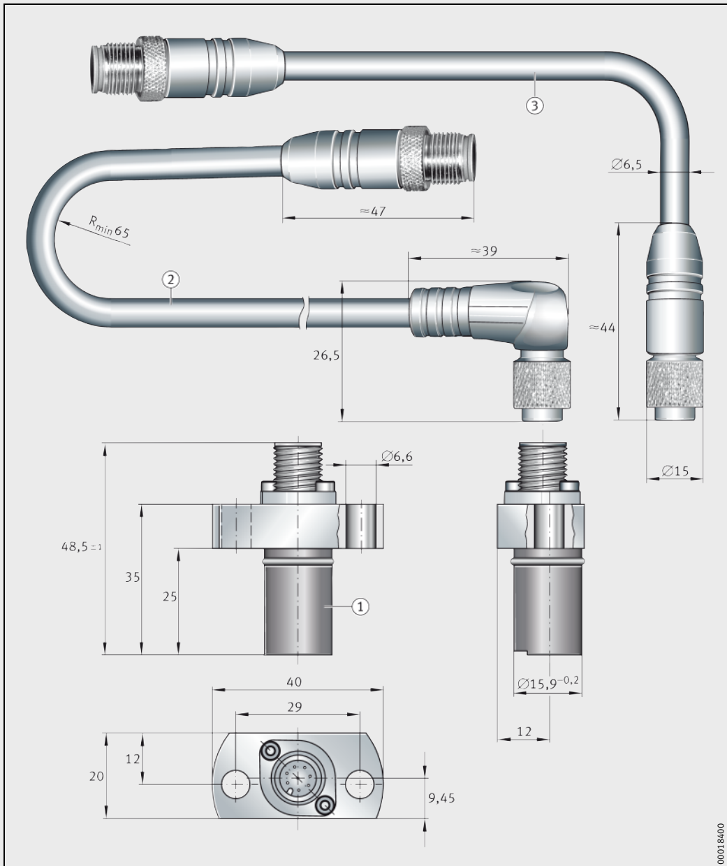
Measuring head 1, connection cable SRMC..-A 2 and SRMC..-S 3. (Design of connection cable: see page 50)
