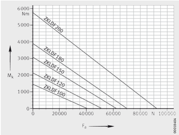
M_k = maximum tilting moment F_a = axial load Figure 8 Static limiting load diagram ZKLDF100 to ZKLDF200
