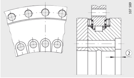
For YRTS325: 2 Screw counterbores open 5)
