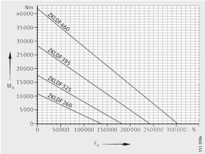
M_k = maximum tilting moment F_a = axial load Figure 9 Static limiting load diagram ZKLDF260 to ZKLDF460
