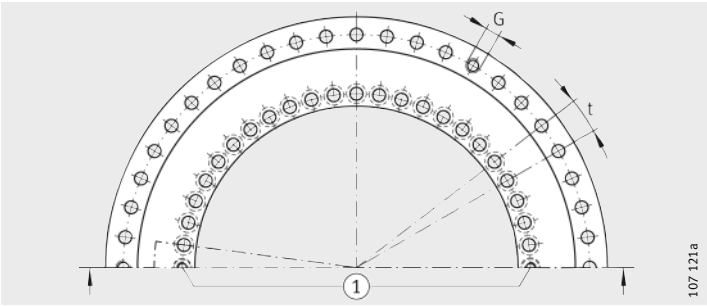
Hole pattern 1 Two retaining screws
