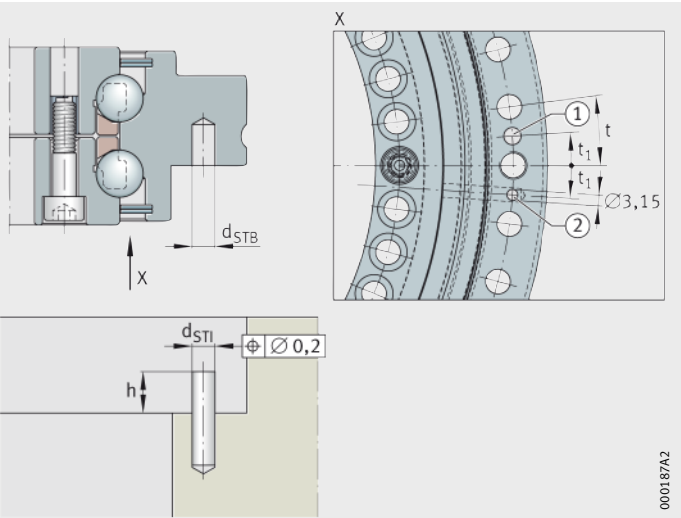
Figure 17 Improved ease of mounting with axial lubrication hole
