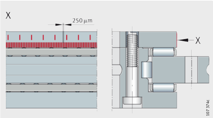
Figure 2 Dimensional scale
