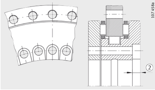
For YRT80-TV and YRT100: 2 Screw counterbores open 5)
