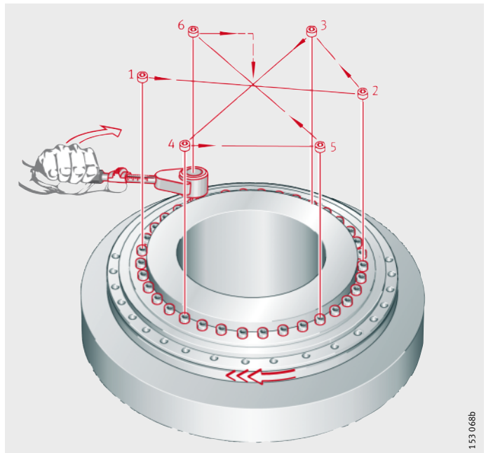
Figure 18 Tightening of fixing screws
